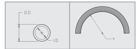
Interlock Sizes: 1-1/2" - 4"
