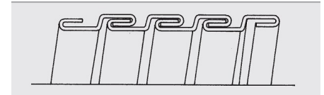
Interlock Sizes: 1-1/2" - 4"
