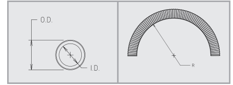
Types ABRH Strip Profile
