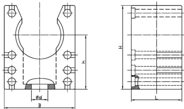
MB Profile
